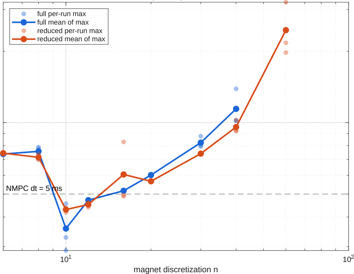
Worst-case per-step solve time vs n
